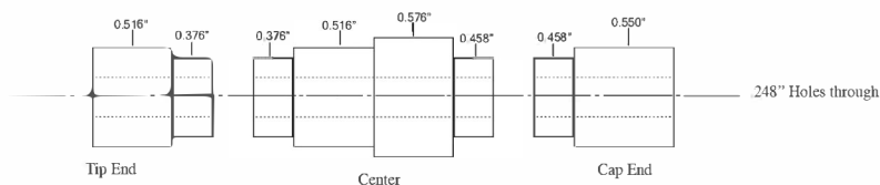
Diagram C / Bushings #PKMAJJRBU
